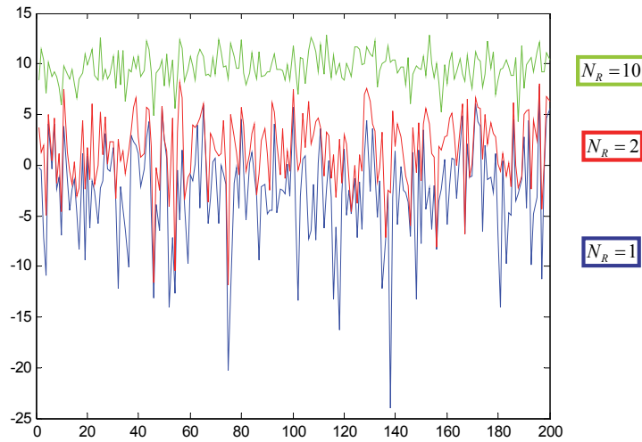
Simulation of 1, 2 & 10 receiver diversity gain
