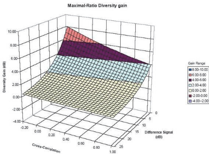
Maximal ratio diversity gain
